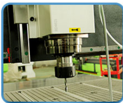
3.5KW air cooling spindle
